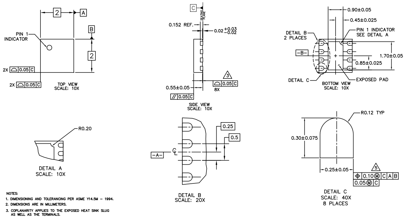
Figure 24. Package Dimensions
