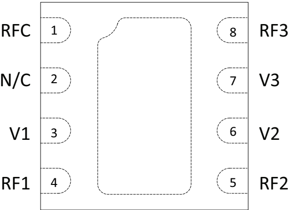
Figure 2. Pinout
