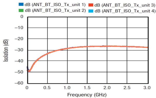
Figure 7. RF1 to RF2 Isolation
