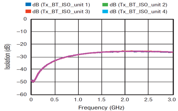
Figure 4. RFC to RF3 Isolation
