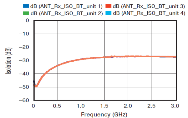
Figure 20. RF3 to RF2 Isolation
