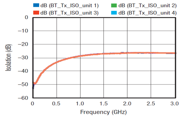
Figure 16. RFC to RF1 Isolation
