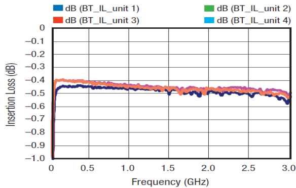
Figure 15. RFC to RF3 Insertion Loss
