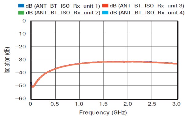
Figure 13. RF2 to RF3 Isolation
