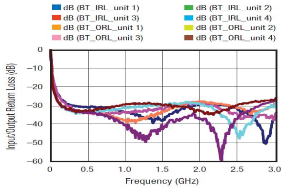
Figure 17. RFC to RF3 Return Loss
