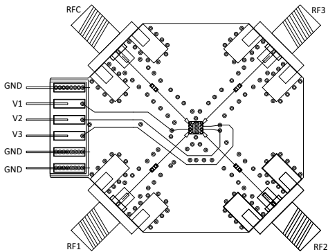
Figure 22. Evaluation Board Assembly Diagram
