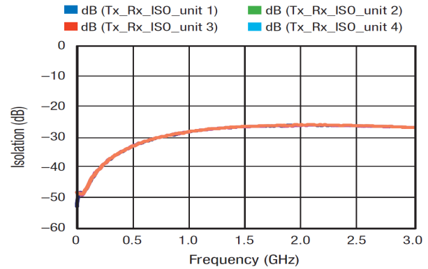
Figure 6. RFC to RF2 Isolation
