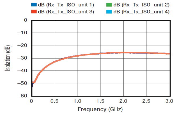
Figure 12. RFC to RF3 Isolation
