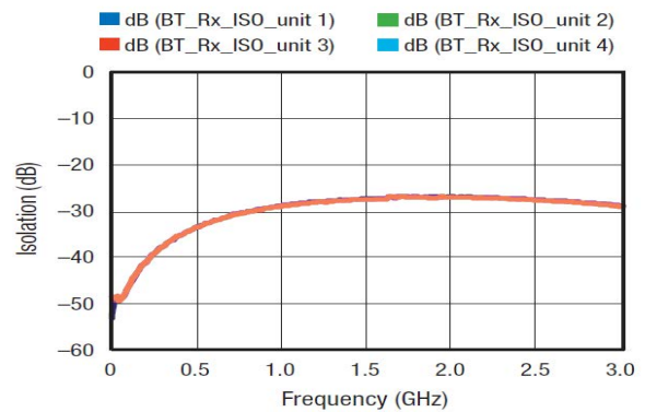
Figure 18. RFC to RF2 Isolation
