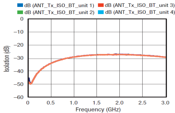
Figure 19. RF3 to RF1 Isolation
