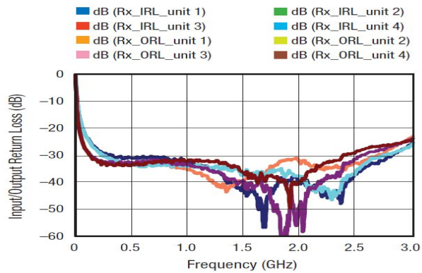
Figure 11. RFC to RF2 Return Loss
