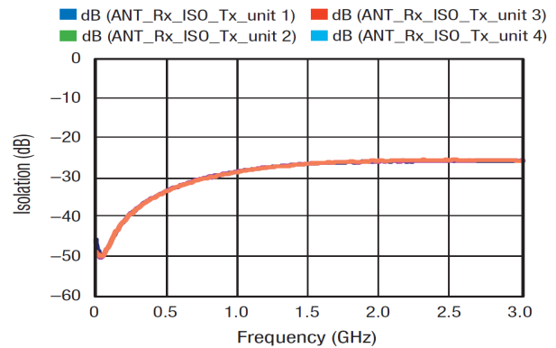
Figure 8. RF1 to RF3 Isolation
