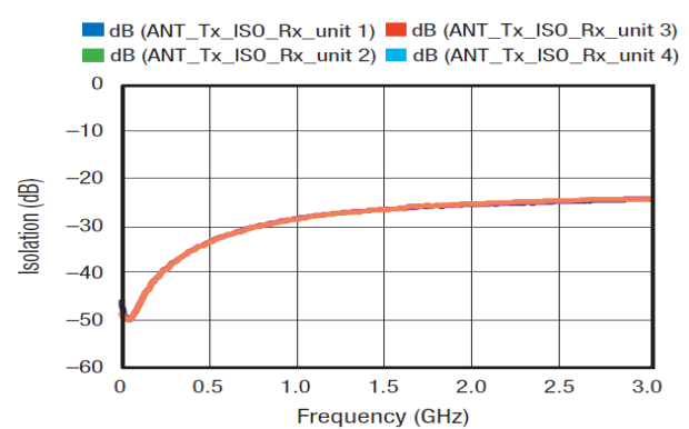
Figure 14. RF2 to RF1 Isolation
