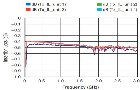
Figure 3. RFC to RF1 Insertion Loss
