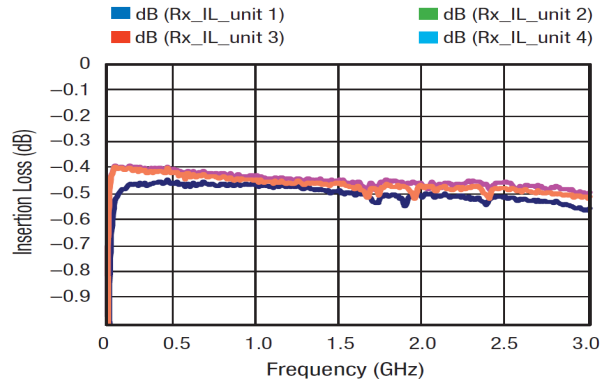
Figure 9. RFC to RF2 Insertion Loss
