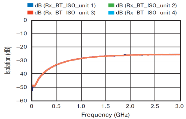
Figure 10. RFC to RF2 Isolation
