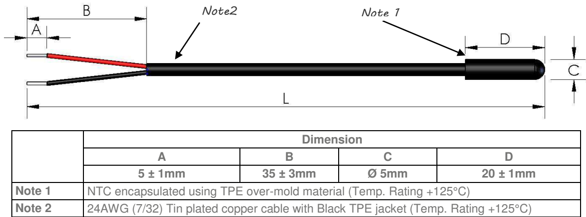
Figure 1: TPE Overmoulded Probe Ø 5 x 20mm
