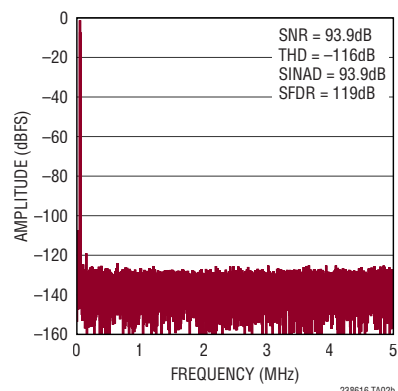
32k Point FFT, f_{\text{SAMPL}} = 10\text{Mps} , f_{\text{IN}} = 50\text{kHz}
