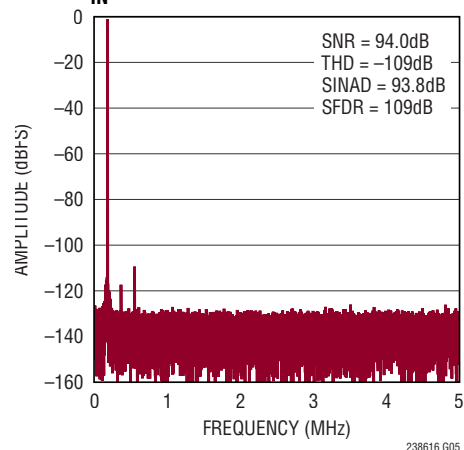
32k Point FFT f_{\text{SAMPL}} = 10\text{Mps} , f_{\text{IN}} = 200\text{kHz}
