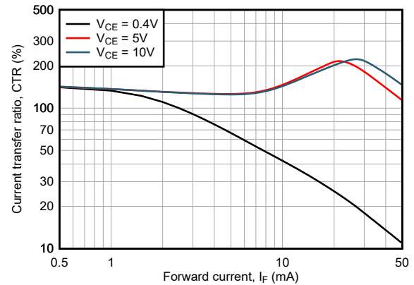
Figure 6-8. Current Transfer Ratio vs Forward Current
