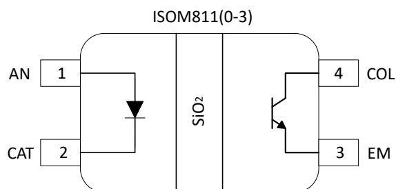
Figure 5-1. ISOM811(0-3) 4-Pin SOIC (Top View)
