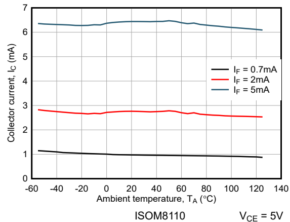
Figure 6-9. Collector Current vs Ambient Temperature
