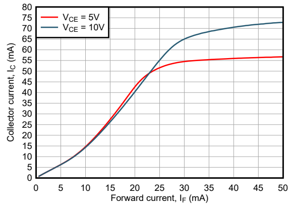
Figure 6-7. Collector Current vs Forward Current
