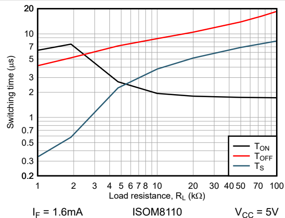
Figure 6-11. Switching Time vs Load Resistance
