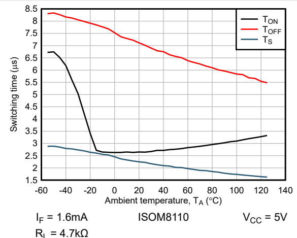
Figure 6-12. Switching Time vs Ambient Temperature
