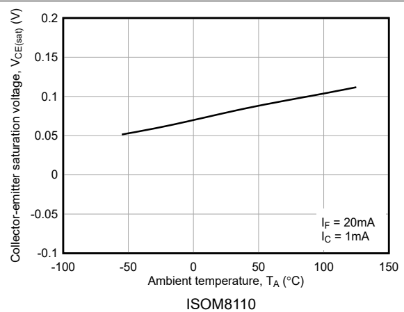
Figure 6-6. Collector-Emitter Saturation Voltage vs Ambient Temperature
