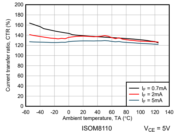
Figure 6-10. Current Transfer Ratio vs Ambient Temperature
