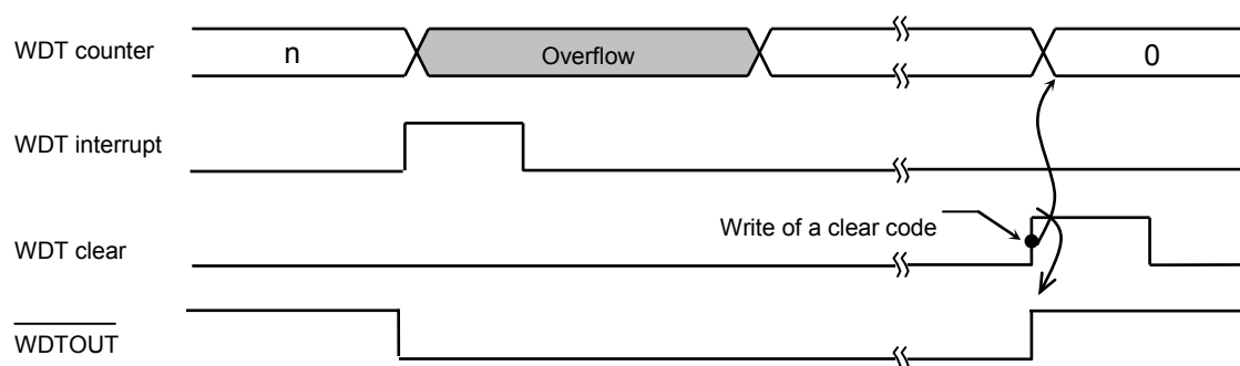
Fig. 16-2 Normal Mode
