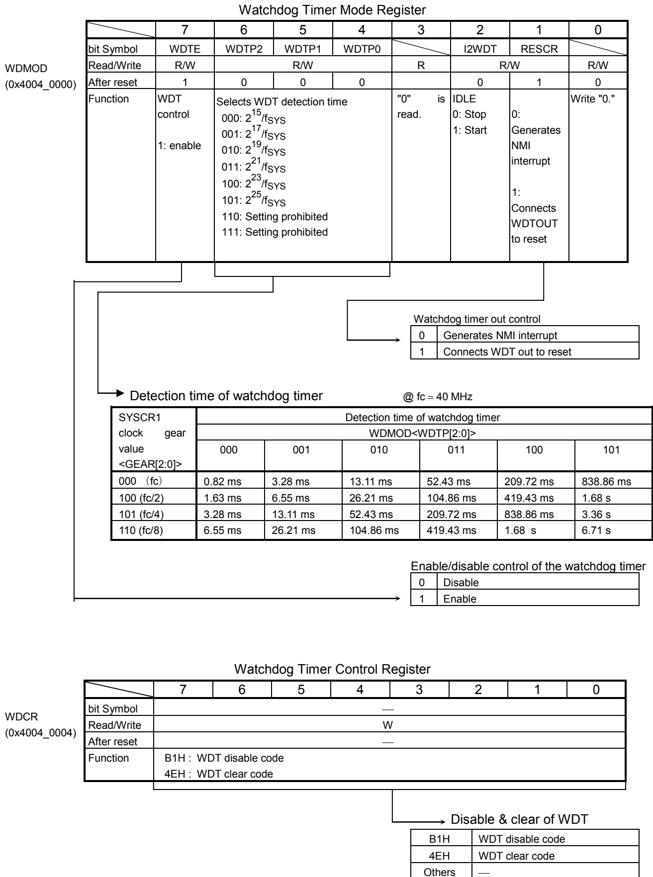
Fig. 16-4 Watchdog Timer Registers
