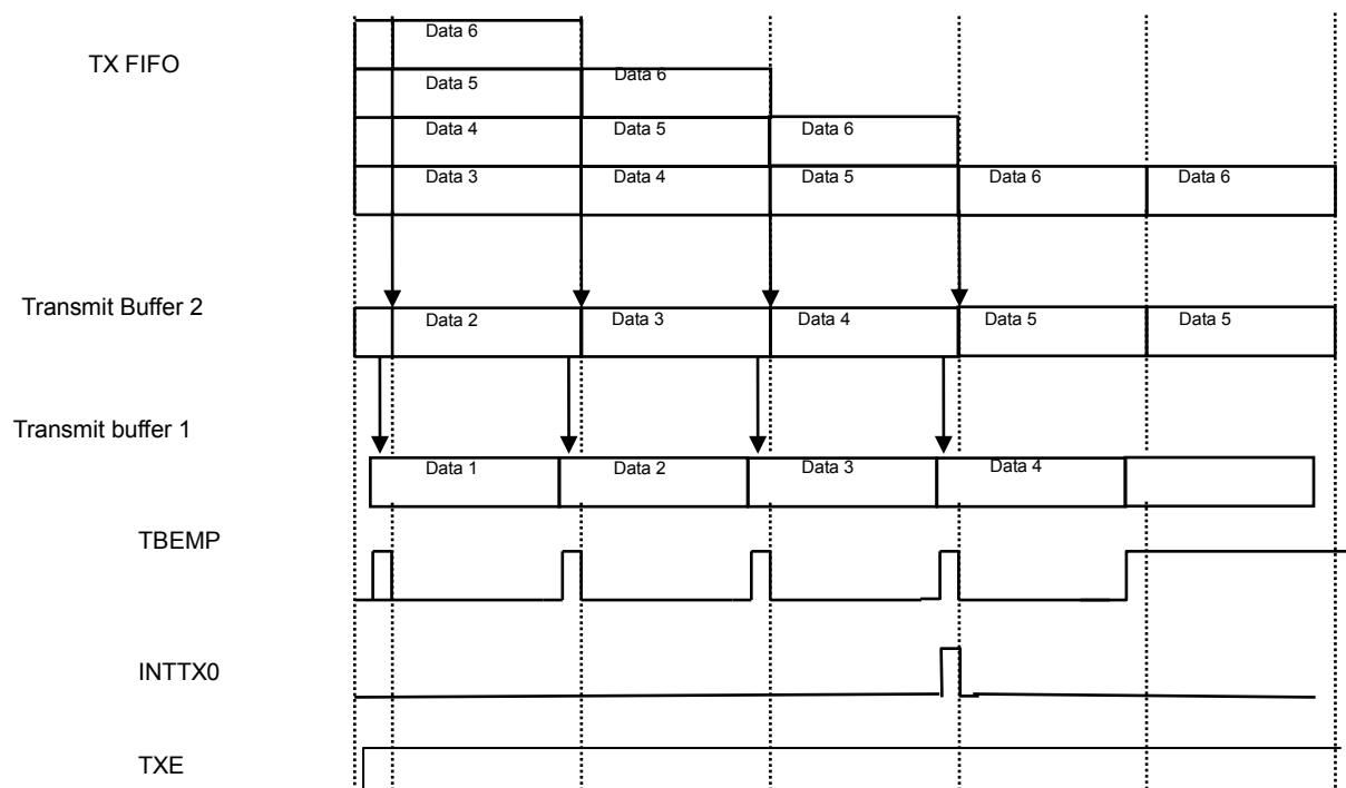
Fig. 11-9 Transmit FIFO Operation
