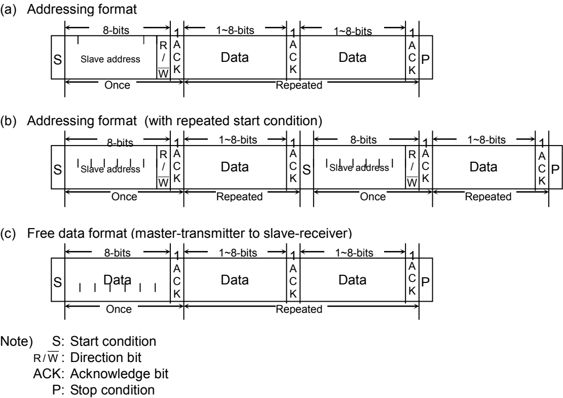
Fig. 12-2 I 2 C Bus Mode Data Formats
