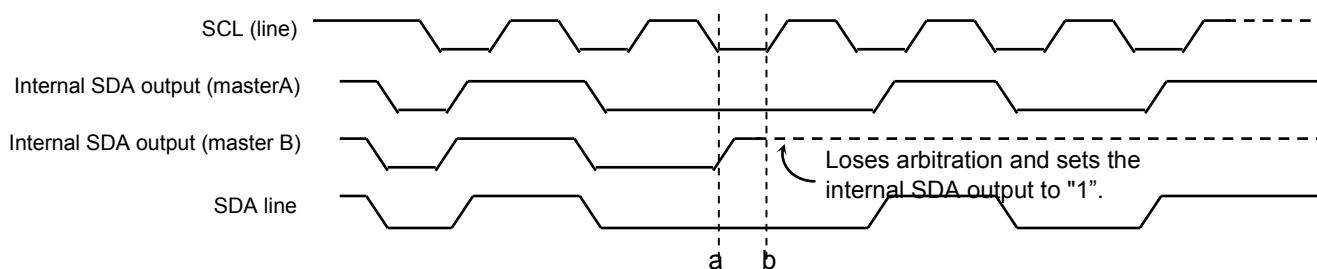
Fig. 12-12 Lost Arbitration
