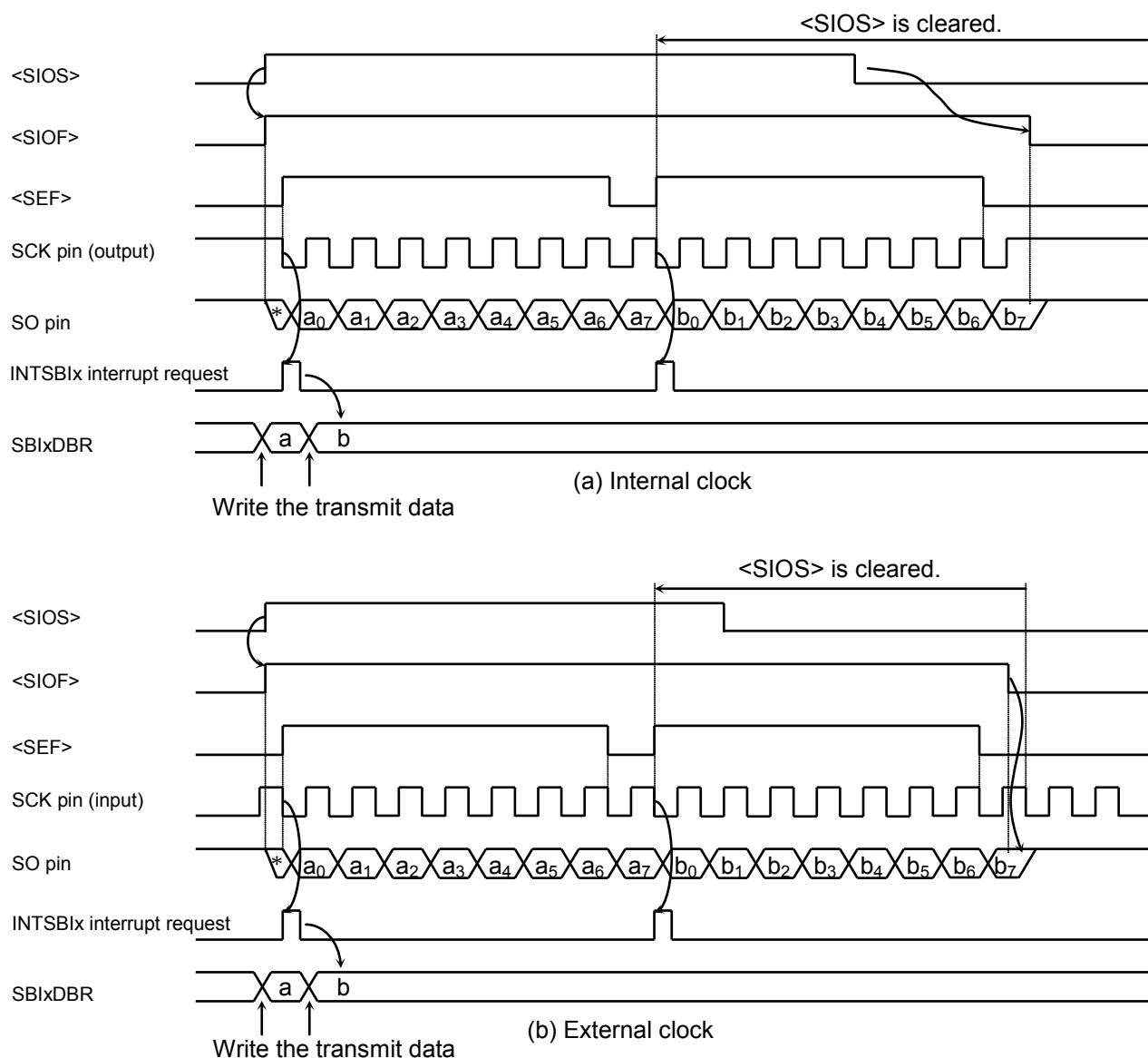
Fig. 12-27 Transmit Mode
