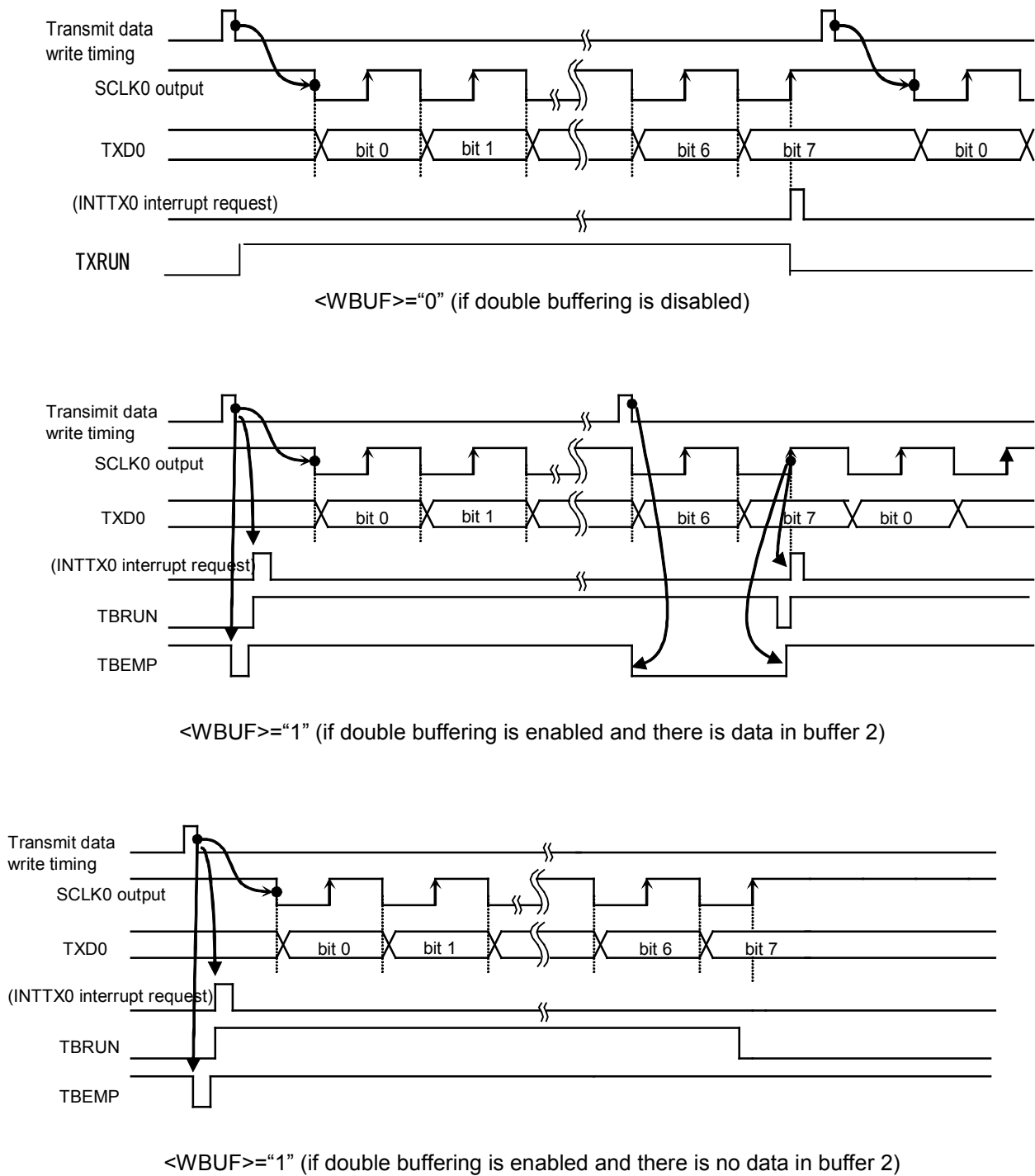
Fig. 11-10 Transmit Operation in the I/O Interface Mode (SCLK0 Output Mode)
