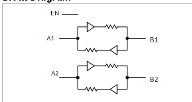
Figure 1: Block Diagram
