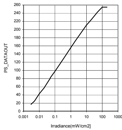
Fig.14 Irradiance – PS_DATAOUT
