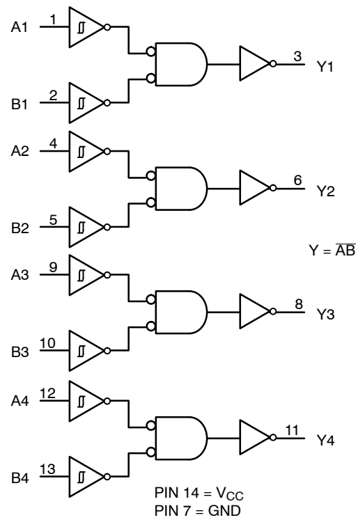
Figure 4. Logic Diagram
