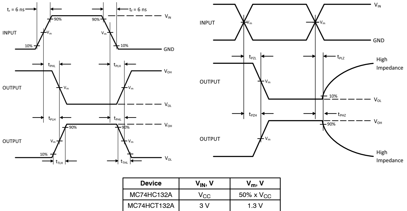
Figure 3. Switching Waveforms
