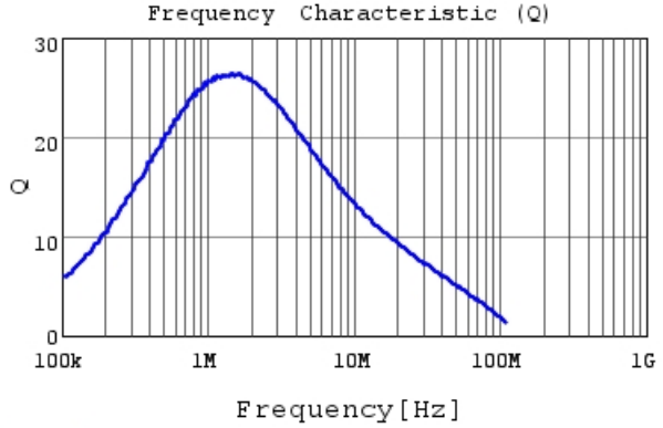
DFE18SANR47MG0 Q
