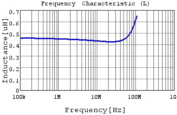
DFE18SANR47MG0 L
