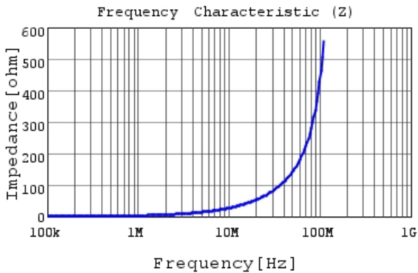
DFE18SANR47MG0 |Z|
