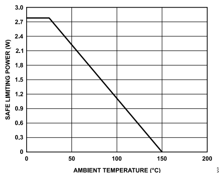
Figure 7. Thermal Derating Curve for 20-Lead Increased Creepage SOIC [SOIC_IC] (RI-20-1), Dependence of Safety Limiting Power with Ambient Temperature per IEC 60747-17
