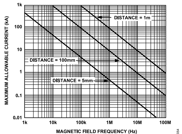
Figure 54. Maximum Allowable Current for Various Current-to-ADuM447x Spacings
