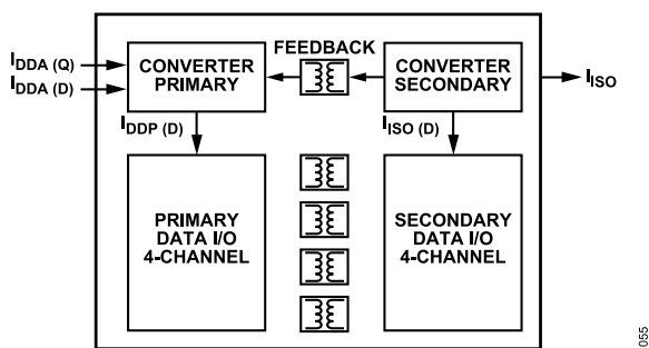
Figure 55. Power Consumption Within the ADuM447x
