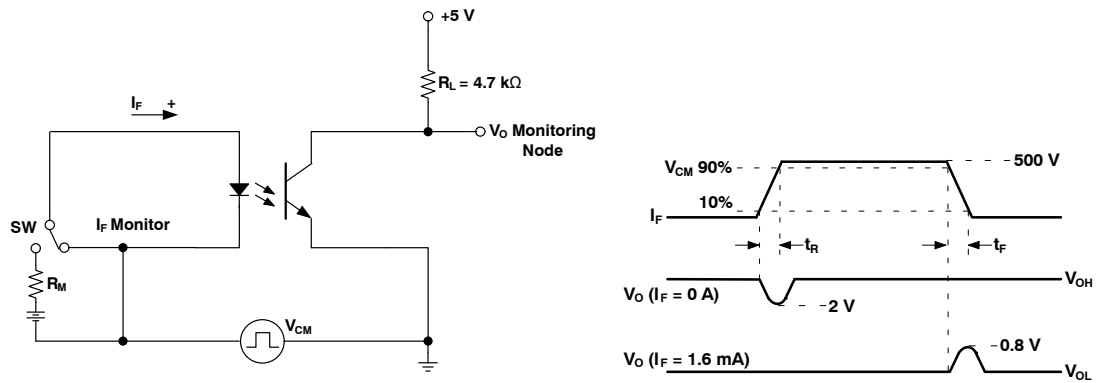
Figure 2. Test Circuit for Instantaneous Common-Mode Rejection Voltage
