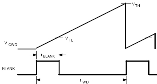
Watchdog-triggered commutation
