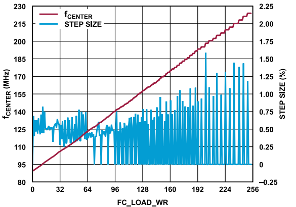
Figure 18. f_{\text{CENTER}} and Step Size vs. FC_LOAD_WR
