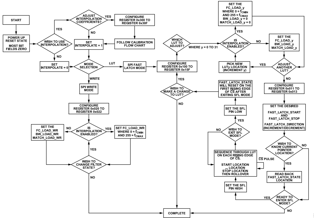
Figure 26. Programming Flowchart
