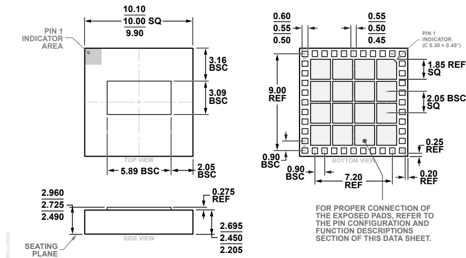
Figure 28. 40-Terminal Land Grid Array [LGA] (CC-40-11) Dimensions shown in millimeters
