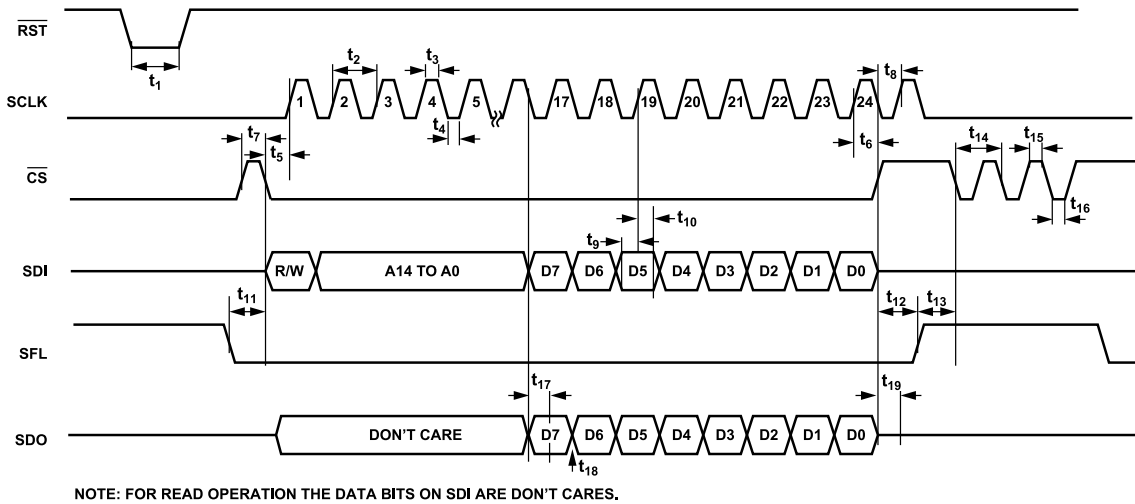
Figure 2. Timing Diagram
