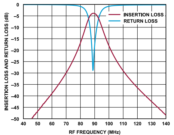
Figure 5. Insertion Loss and Return Loss vs. RF Frequency for Nominal Bandwidth at 90 MHz
