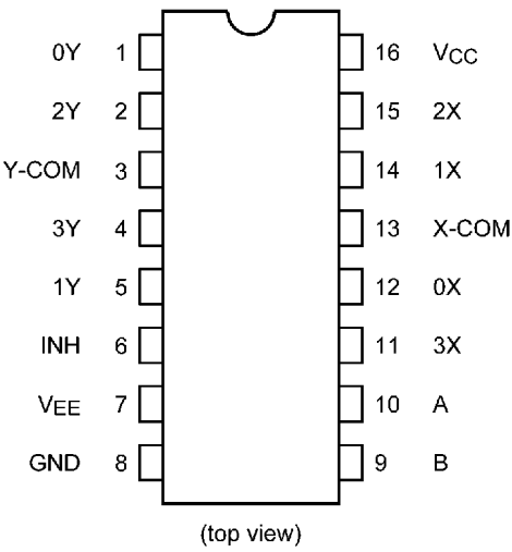
74HC4052FT
