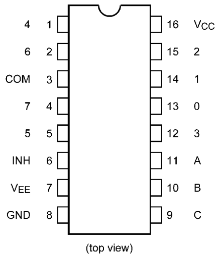
74HC4051FT
