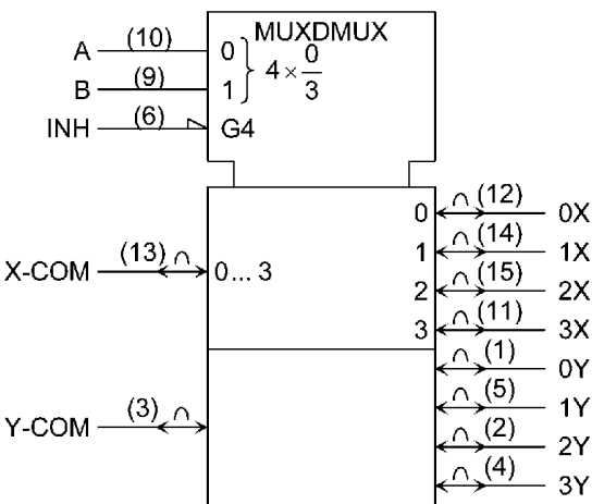
74HC4052FT
