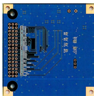
(b) THEVAF(R)84C (Bottom Side)
