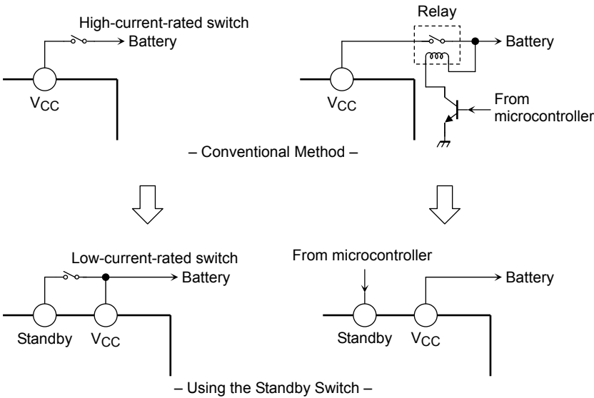
Figure 2 Standby Switch
