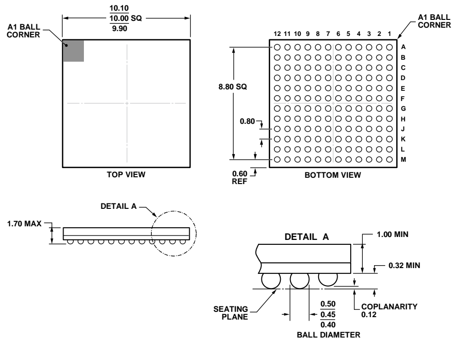
COMPLIANT TO JEDEC STANDARDS MO-275-EEAB-1. Figure 44. 144-Ball Chip Scale Package Ball Grid Array [CSP_BGA] (BC-144-7) Dimensions shown in millimeters
