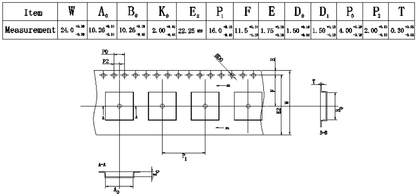
Figure 10. CYBLE-222005-00 Tape Dimensions
