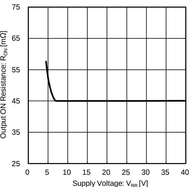
Figure 13. Output ON Resistance vs Supply Voltage
