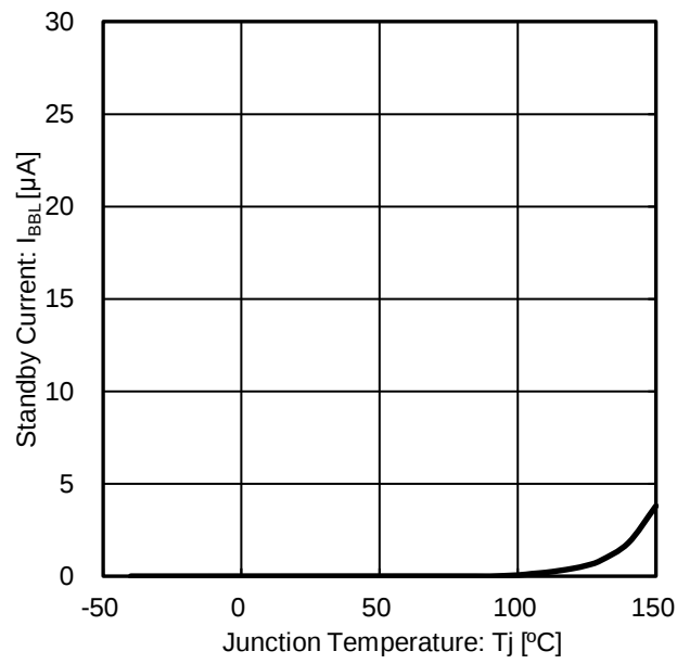
Figure 7. Standby Current vs Junction Temperature
