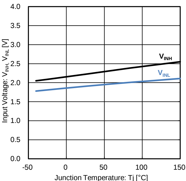
Figure 11. Input Voltage vs Junction Temperature
