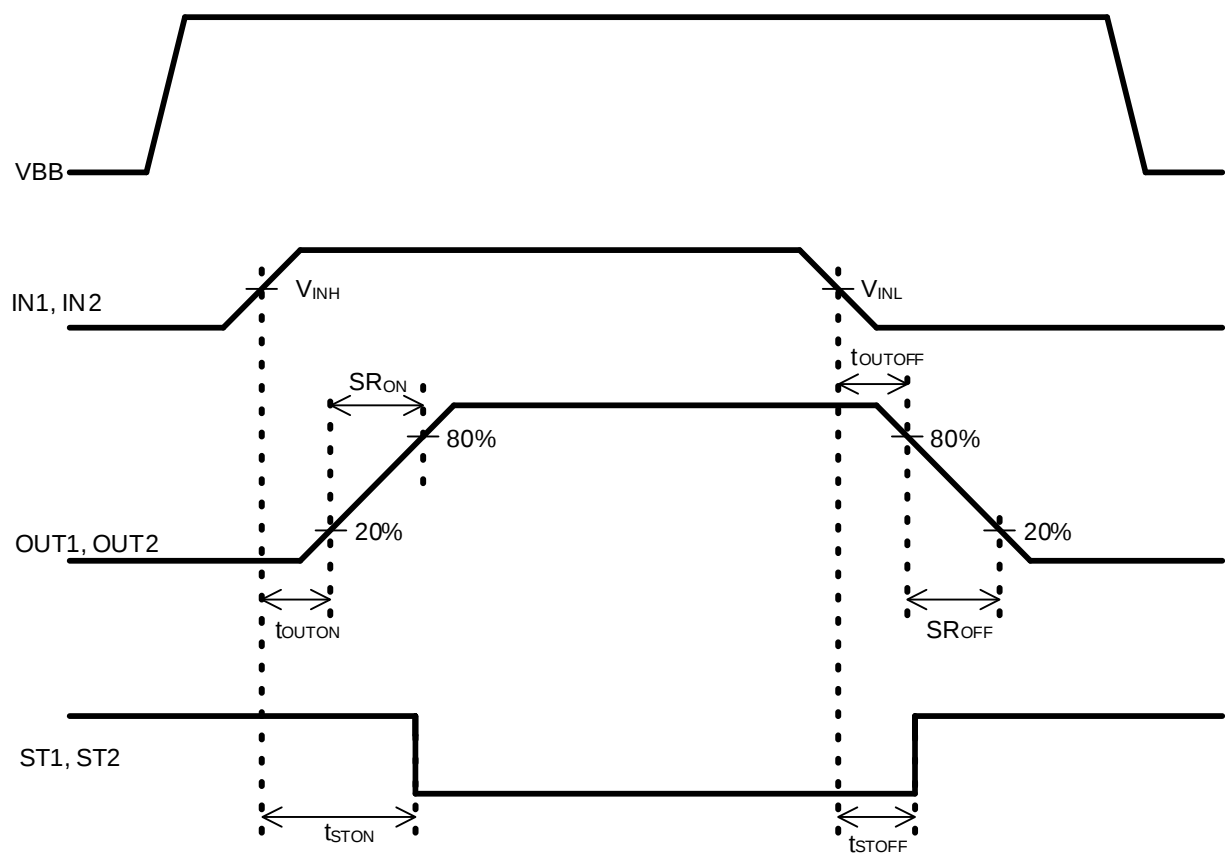
Figure 32. Timing Chart
