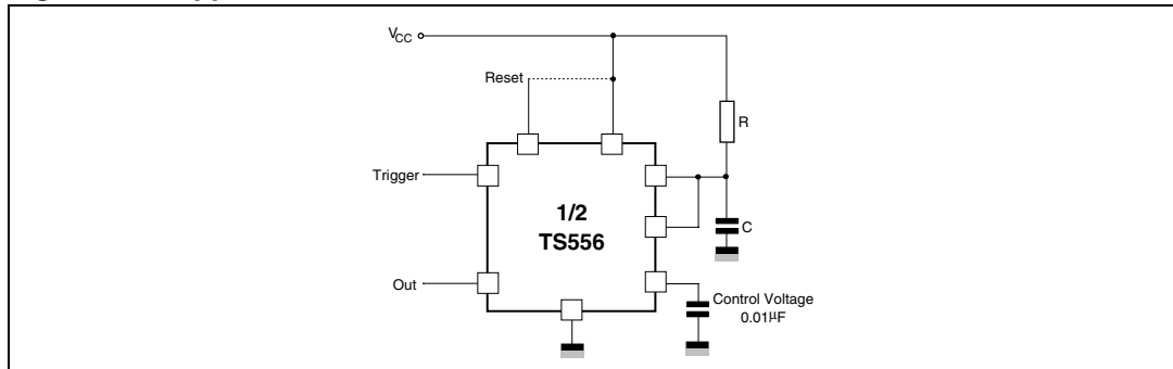
Figure 4. Application schematic
