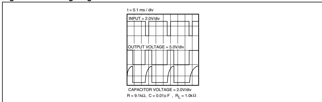
Figure 5. Timing diagram
