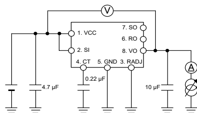
Measurement Circuit for Figure 9
