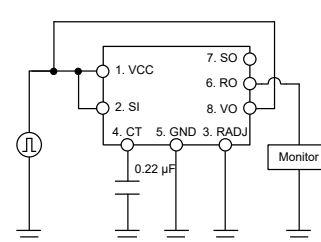
Measurement Circuit for Figure 13, 14
