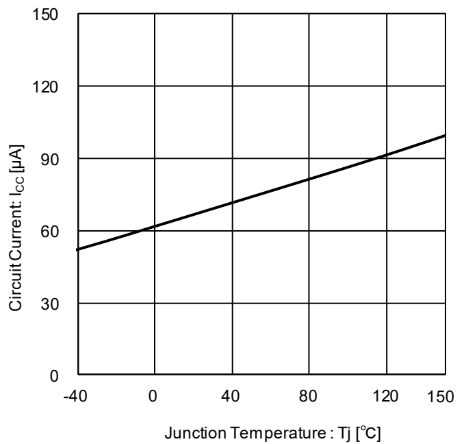
Figure 6. Circuit Current vs. Junction Temperature
