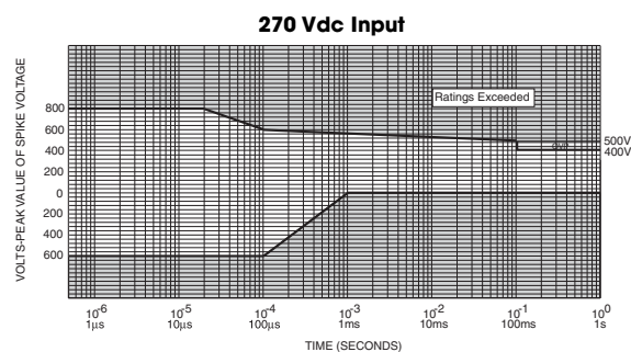
Figure 2 — Long term safe operating area curves; 1% duty cycle maximum, for short duration transient capability refer to specifications
