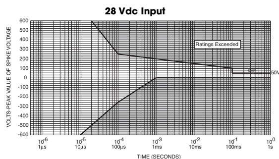
Figure 2 — Long term safe operating area curves; 1% duty cycle maximum, for short duration transient capability refer to specifications
