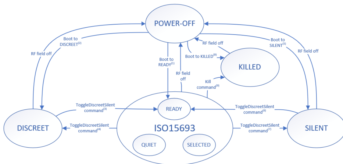
Figure 10. ST25TVxxxC state transition diagram
