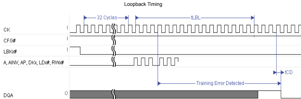
Figure 15. Loopback Timing
