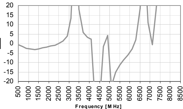
Phase Balance
