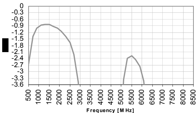
Insertion Loss
