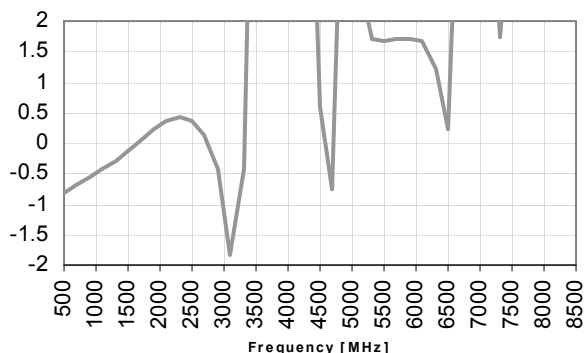
Amplitude Balance
