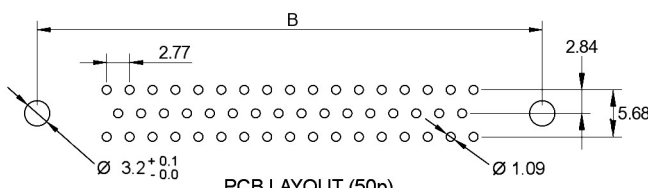
PCB LAYOUT (50p)
