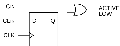
Figure 2. Look-Ahead-Carry Input Structure
