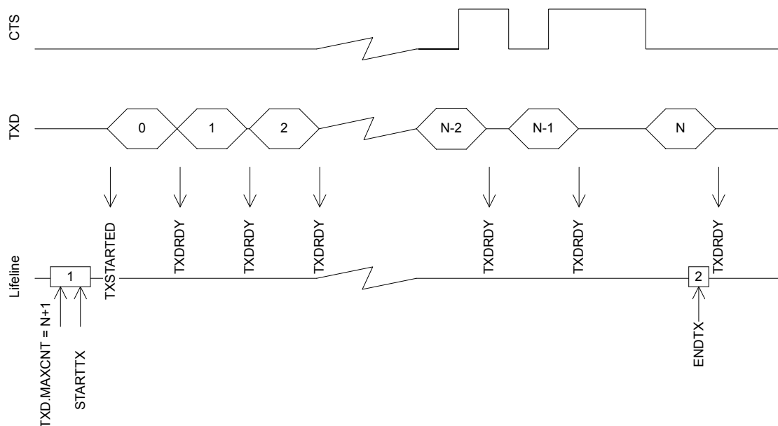
Figure 134: UARTE transmission
