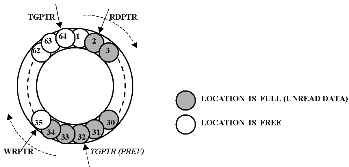
Figure 31. Circular Buffer
