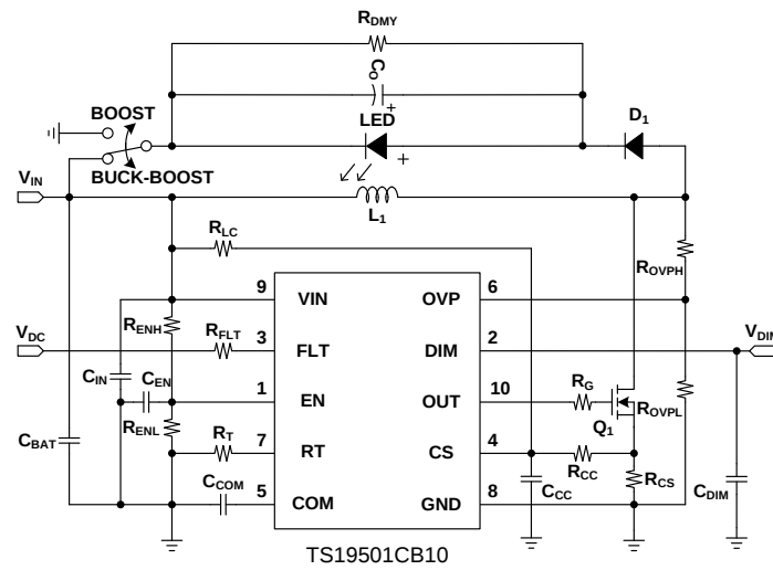
Buck-Boost Regulator
