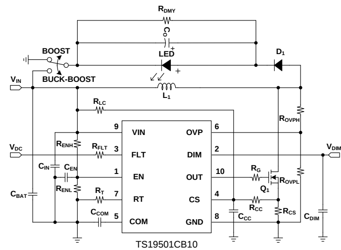
Boost Regulator
