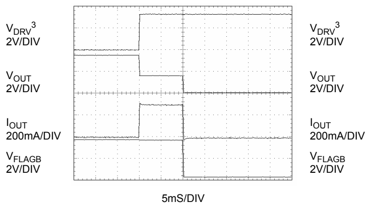
Figure 15. T_{BLANK} Response
