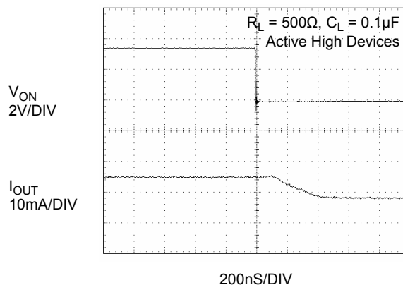
Figure 18. T_{OFF} Response
