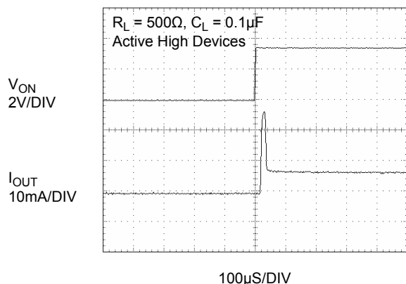
Figure 17. T_{ON} Response
