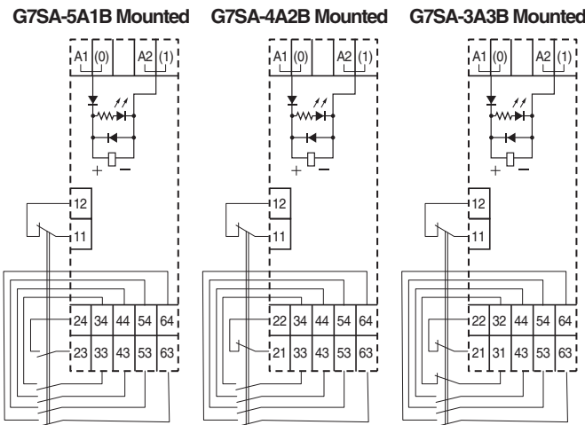
Terminals Arrangement/Internal Connections Diagram (Top View)
