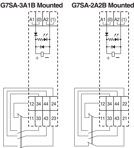
Terminals Arrangement/Internal Connections Diagram (Top View)
