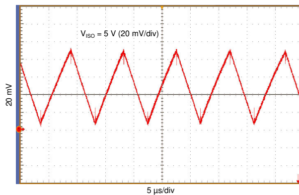
V_{CC} = 5\text{ V} V_{ISO} = 5\text{ V} Figure 7-22. V_{ISO} Ripple Voltage at 130 mA
