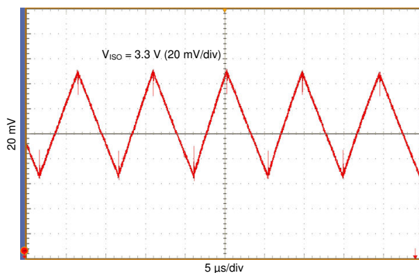
V_{CC} = 5\text{ V} V_{ISO} = 3.3\text{ V} Figure 7-23. V_{ISO} Ripple Voltage at 130 mA
