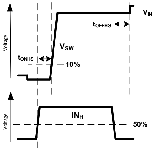
Fig. 3. Propagation Delay Hard Switching t_{\text{ONHS/OFFHS}}
