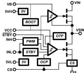
Simplified schematic
