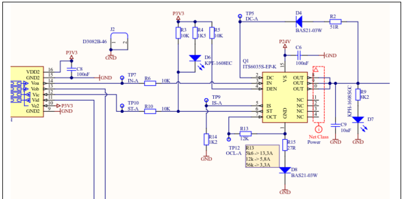
Figure 9 Schematic Power output stage (1 channel)
