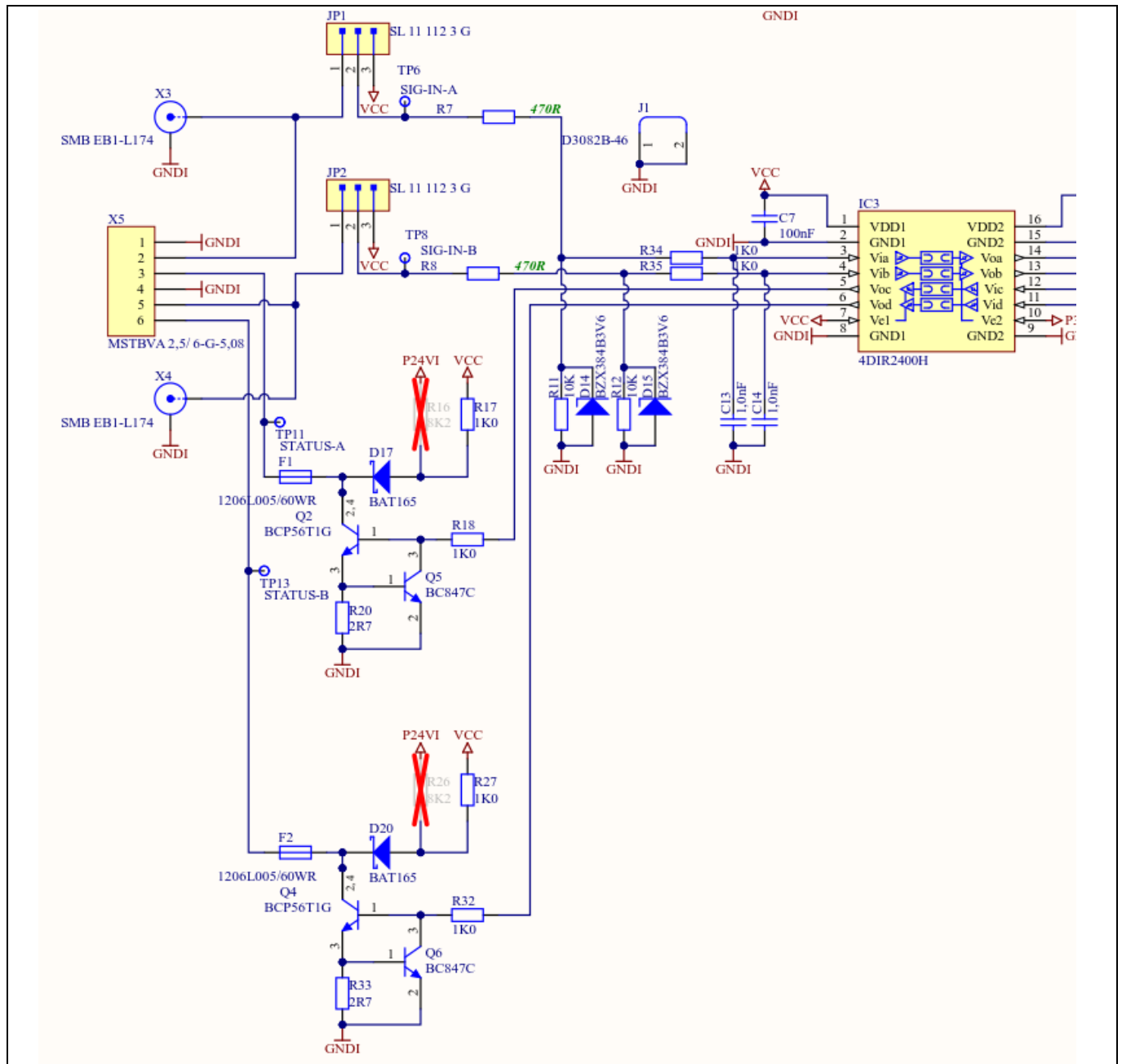
Figure 7 Signal conditioning
