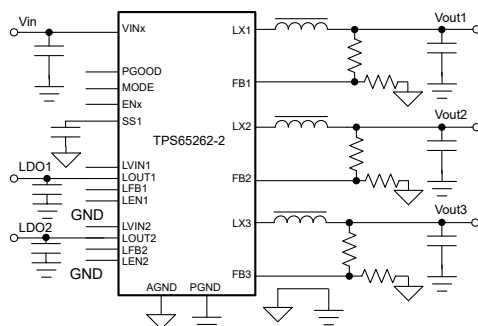
Application Schematic
