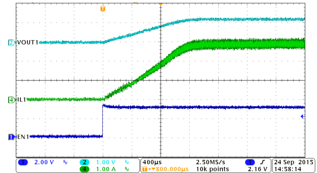
Figure 8-28. PWM Mode, Buck1, Soft-Start with Full Load
