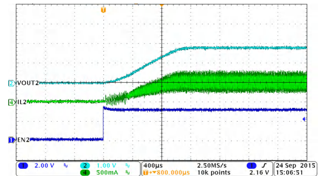
Figure 8-30. PWM Mode, Buck2, Soft-Start with Full Load
