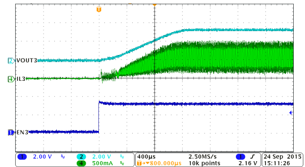
Figure 8-32. PWM Mode, Buck3, Soft-Start with Full Load
