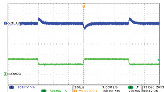
Figure 8-20. Buck3, Load Transient, 0.5 to 0.75 A SR = 0.25 A/µs
