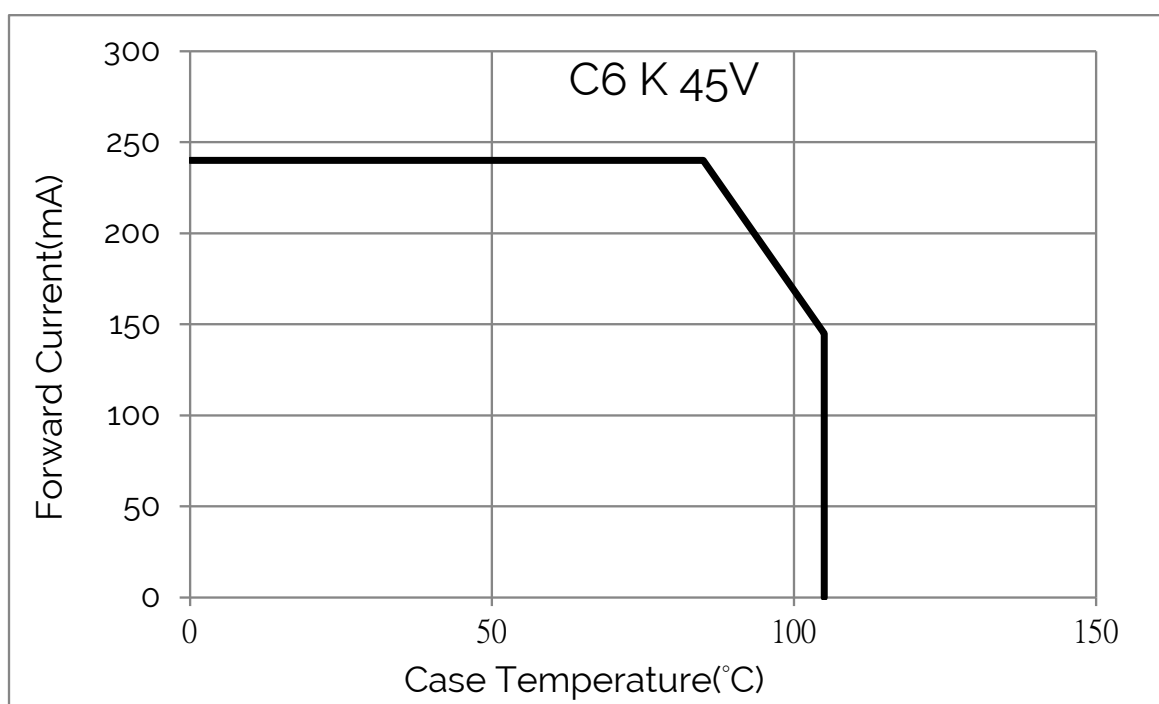
Figure 19: Operating Limits
