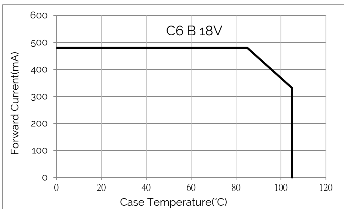
Figure 17: Operating Limits
