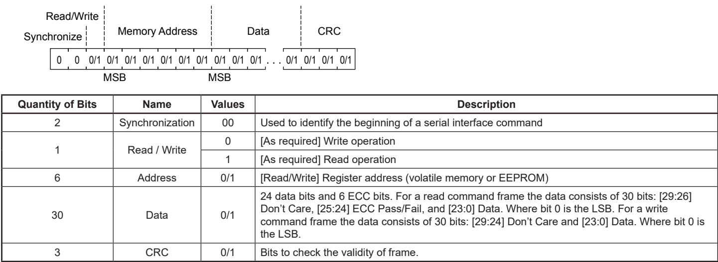
Figure 14: Command Frame General Format
