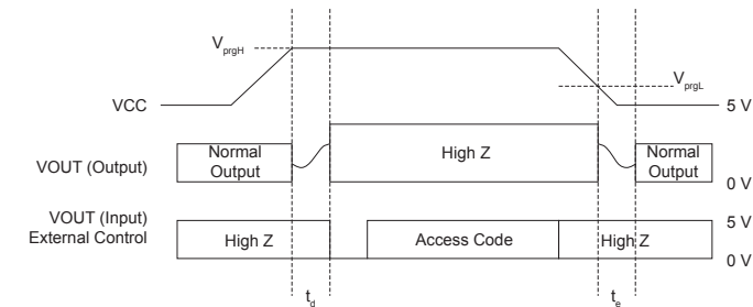
Figure 16: Write Access Code
