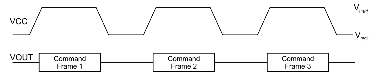
Figure 15: Format for Sending Multiple Transactions
