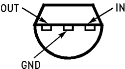
Figure 5. TO-92 Plastic Package Bottom View
