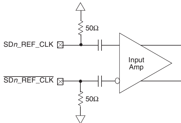
Figure 14-2. Receiver of SerDes Reference Clocks
