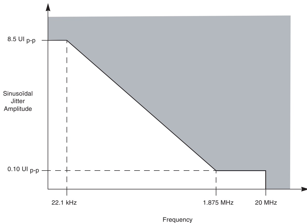
Figure 16-3. Single Frequency Sinusoidal Jitter Limits
