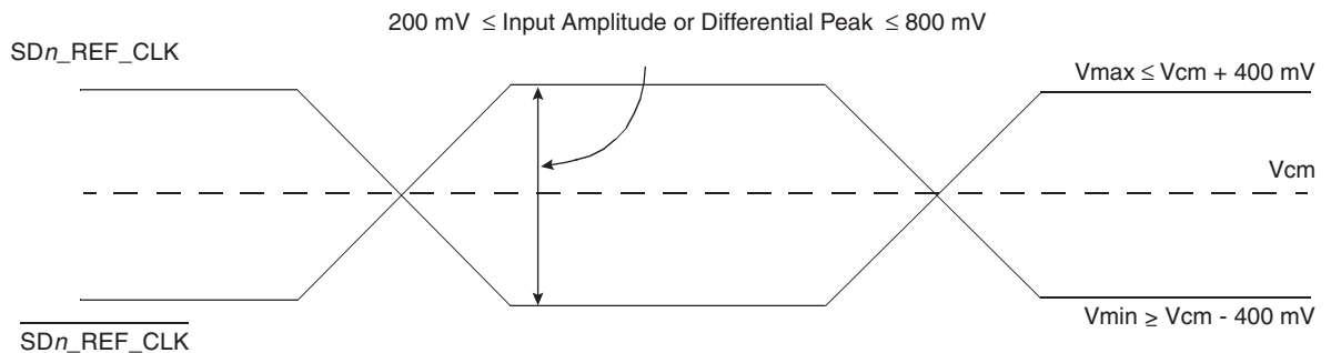
Figure 14-4. Differential Reference Clock Input DC Requirements (External AC-Coupled)
