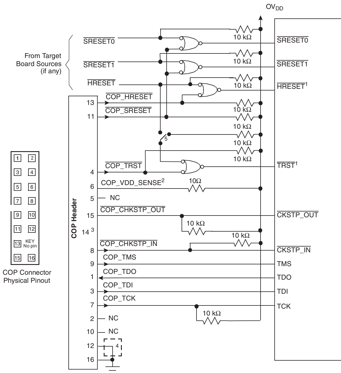
Figure 21-6. JTAG/COP Interface Connection for one PC8640 device
