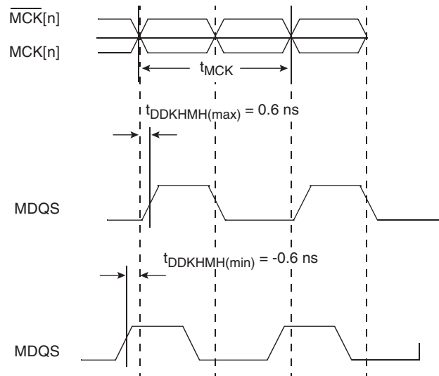
Figure 7-2. Timing Diagram for t_{DDKMHM}
