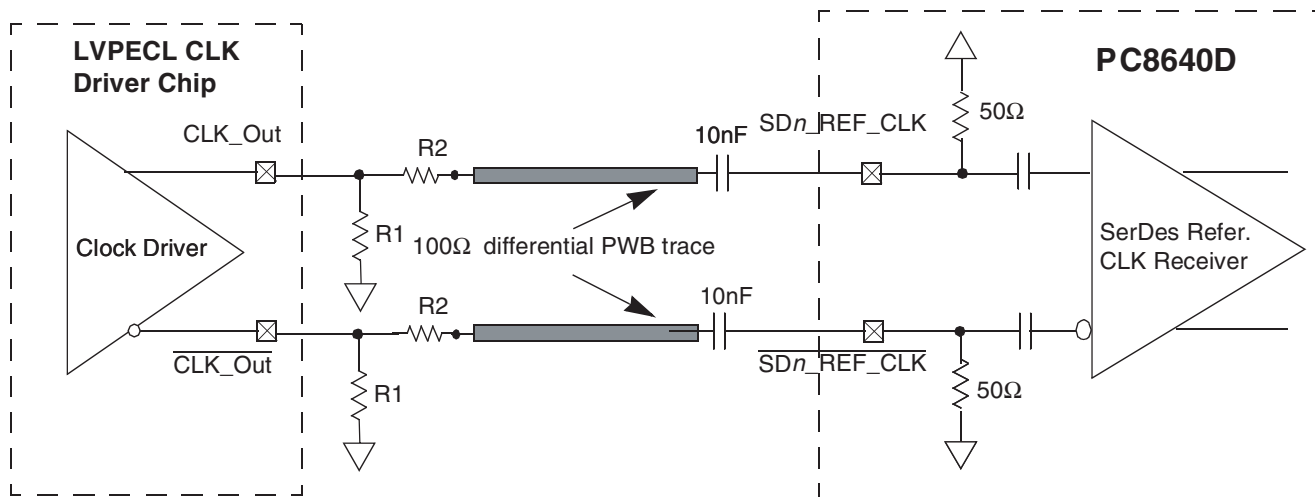
Figure 14-8. AC-Coupled Differential Connection with LVPECL Clock Driver (Reference Only)
