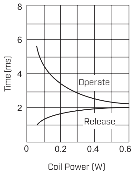
Time Curve
