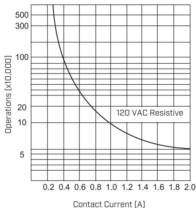
Life Curve
