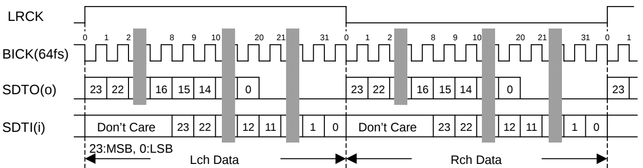
Figure 5. Mode 4 Timing
