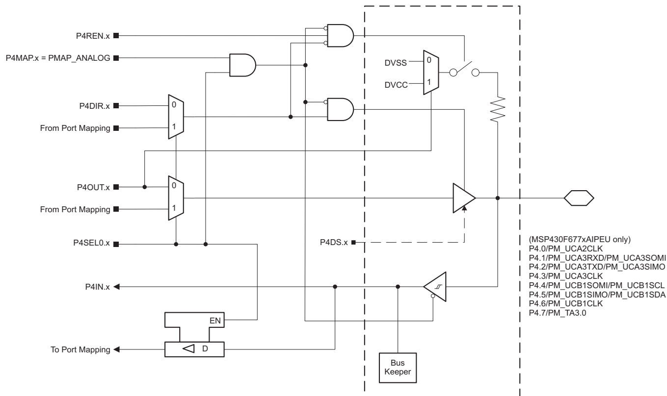
Figure 6-17. Port P4 (P4.0 to P4.7) Diagram (PEU Package Only)
