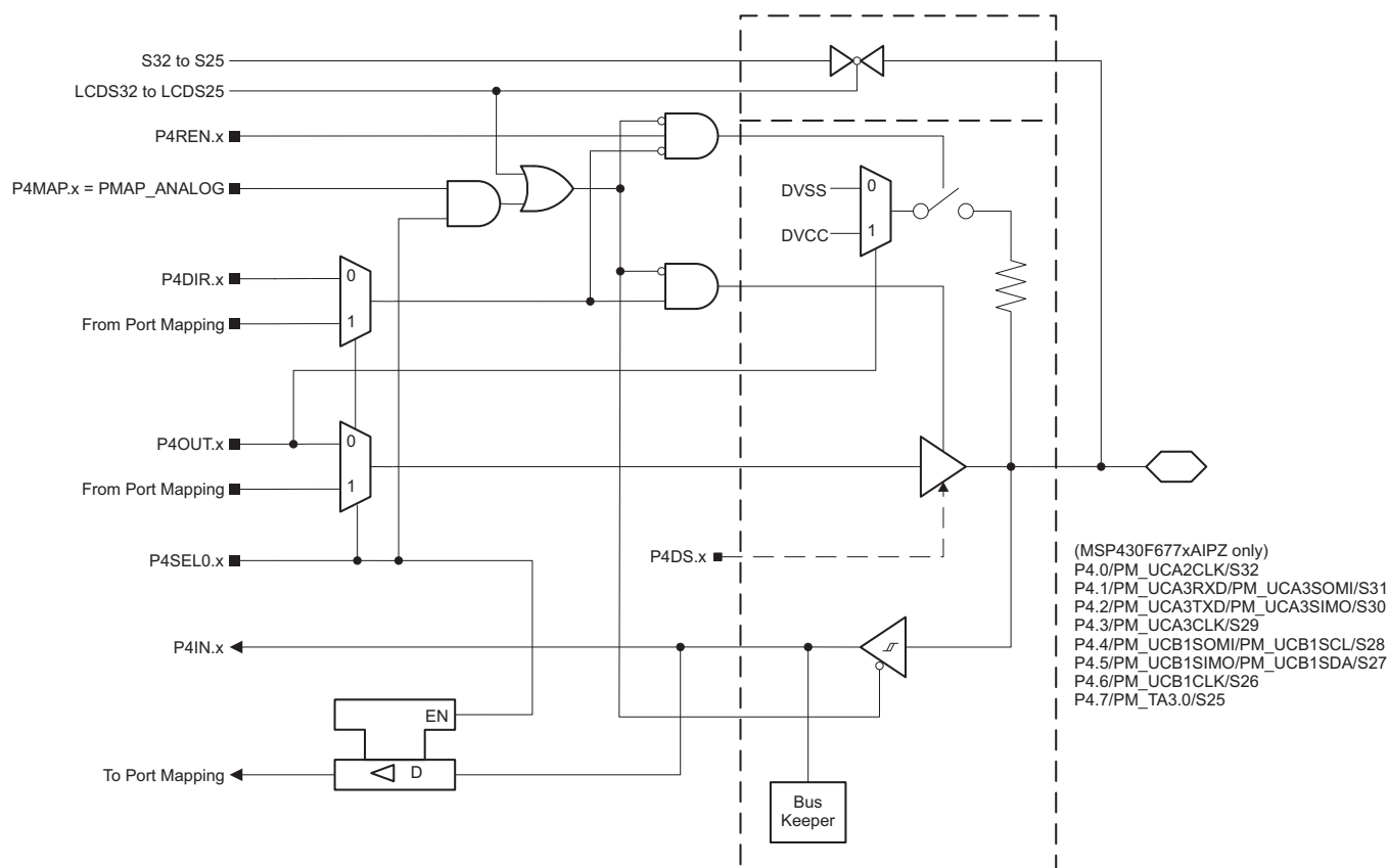
Figure 6-18. Port P4 (P4.0 to P4.7) Diagram (PZ Package Only)
