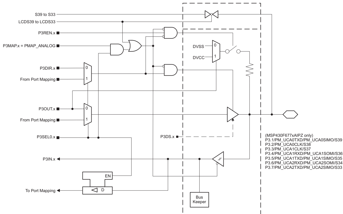
Figure 6-16. Ports P3 (P3.1 to P3.7) Diagram (PZ Package Only)
