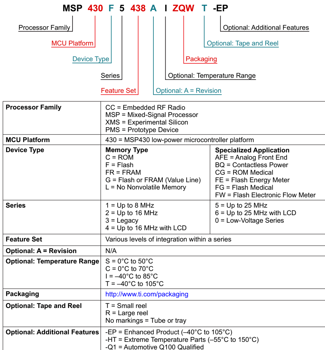
Figure 8-1. Device Nomenclature
