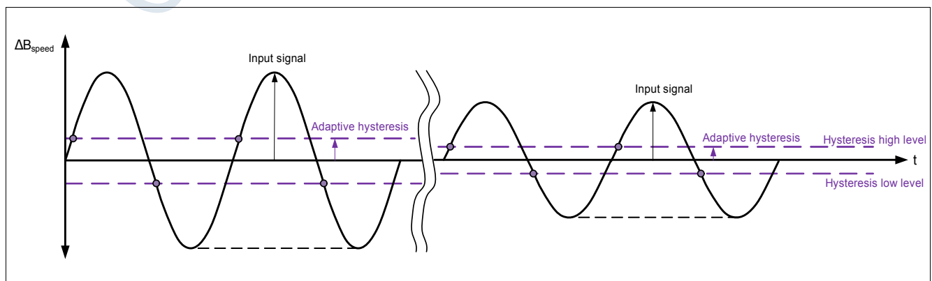
Figure 5 Adaptive Hysteresis
