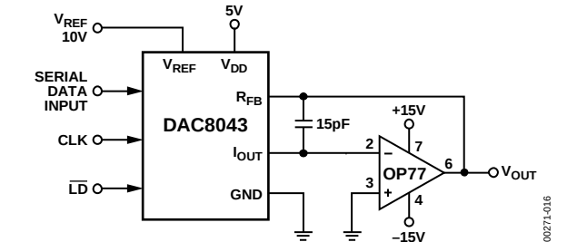
Figure 16. Unipolar Operation with High Accuracy Op Amp (2-Quadrant)
