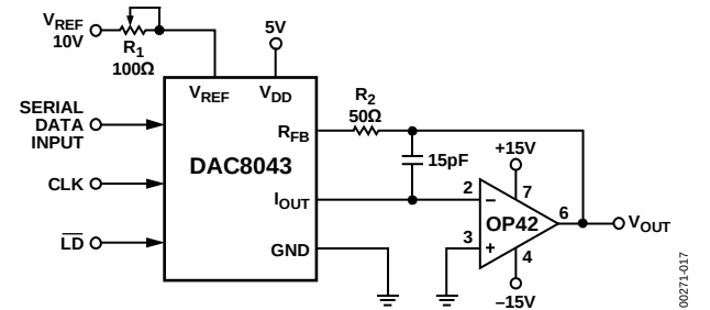
Figure 17. Unipolar Operation with Fast Op Amp and Gain Error Trimming (2-Quadrant)
