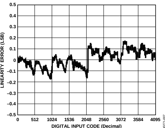
Figure 7. Linearity Error vs. Digital Input Code
