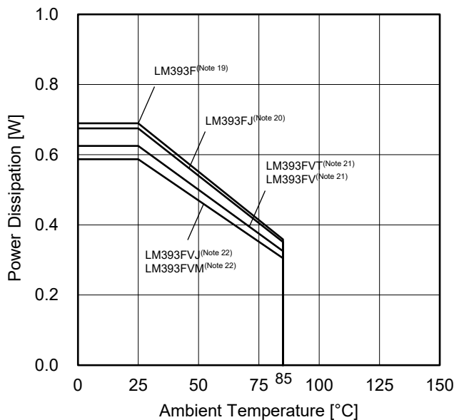
(c) LM393xxx*1
