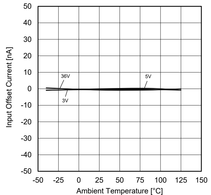
Figure 31. Input Offset Current vs Ambient Temperature
