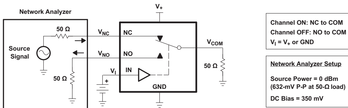
Figure 22. Crosstalk ( X_{TALK} )
