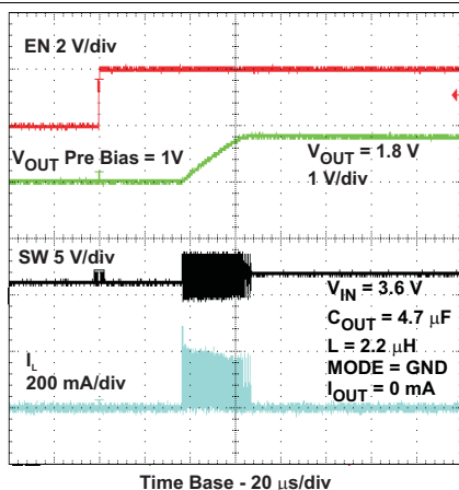
Figure 33. Start-Up in 1-V Prebiased Output – TPS62231
