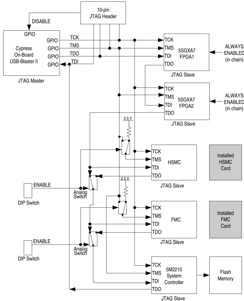
Figure 2-3. JTAG Chain
