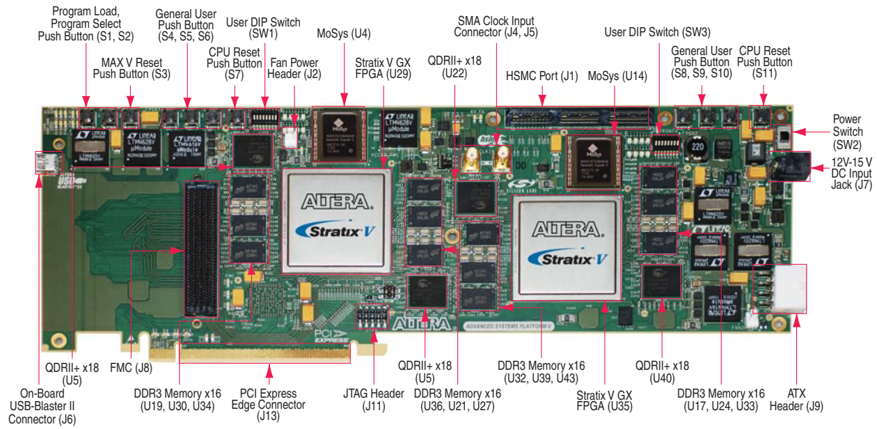
Figure 2–1. Overview of the Stratix V Advanced Systems Development Board Features
