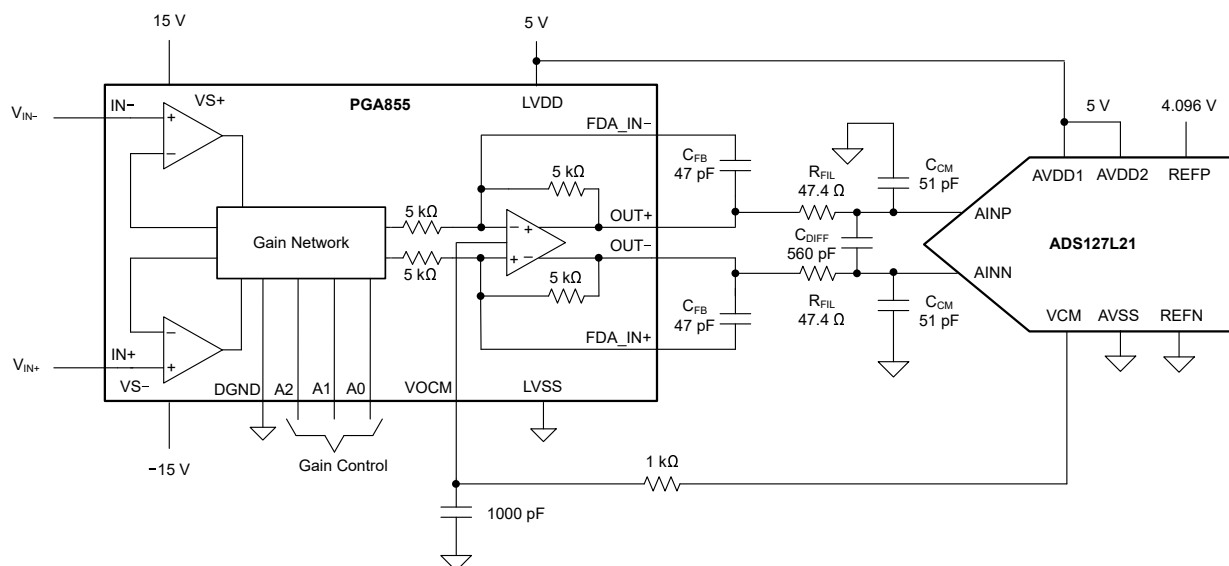
Figure 9-4. PGA855 Driver Circuit
