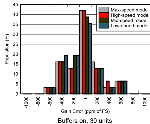
Figure 5-52. Gain Error Distribution
