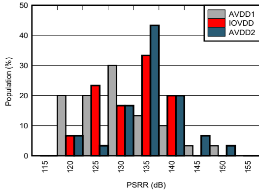
Figure 5-79. DC PSRR Distribution
