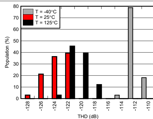
Figure 5-58. THD Distribution
