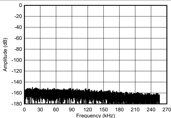
Sinc4 filter
