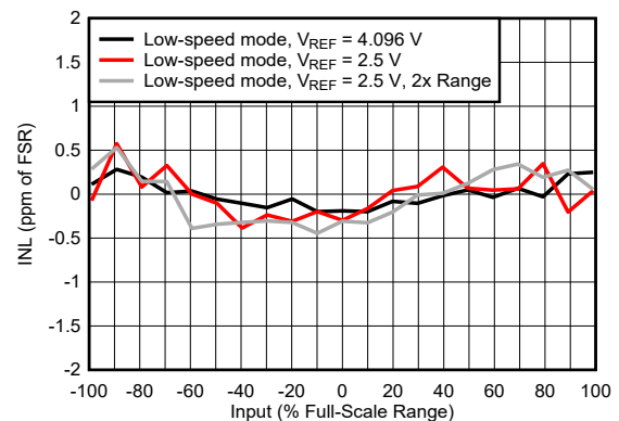
Figure 5-64. INL Error vs Input Voltage
