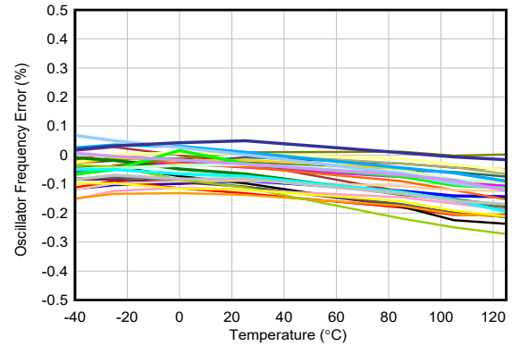
Figure 5-74. Oscillator Frequency vs Temperature
