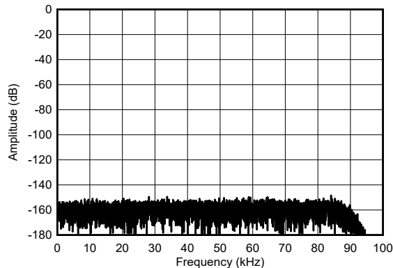
Figure 5-19. Mid-Speed Mode, Shorted-Input FFT
