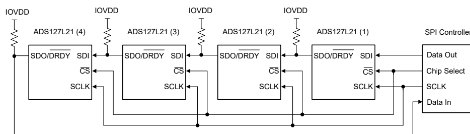
Figure 7-42. Daisy-Chain Connection
