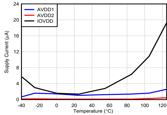
Figure 5-88. Power-Down Mode Supply Current vs Temperature
