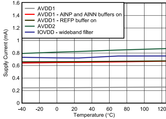
Figure 5-85. Power-Supply Current vs Temperature
