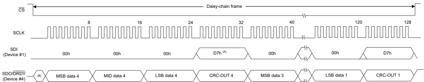
Figure 7-45. Read Conversion Data in Daisy-Chain Connection
