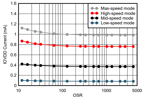
Figure 5-87. IOVDD Current vs Oversampling Ratio
