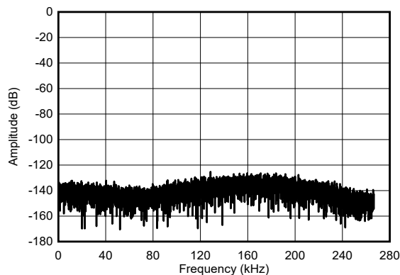
Figure 5-21. Mid-Speed Mode, Shorted-Input FFT
