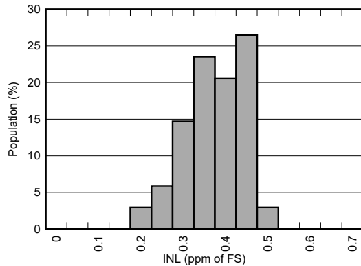
Figure 5-67. INL Distributions
