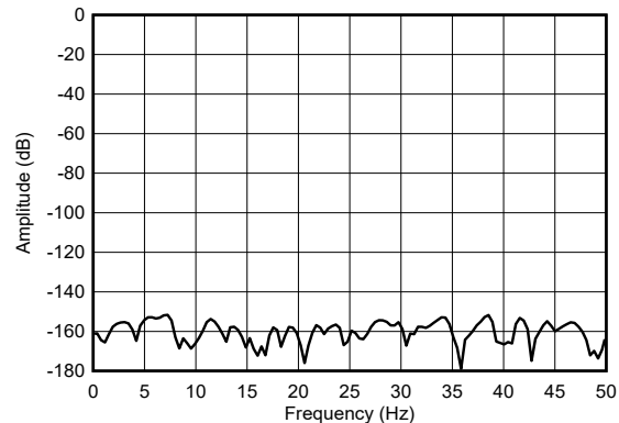
Figure 5-20. Mid-Speed Mode, Shorted-Input FFT
