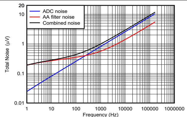
Figure 9-12. Total Noise
