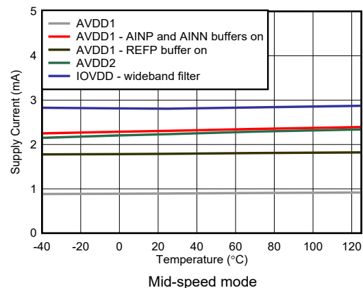
Figure 5-84. Power-Supply Current vs Temperature
