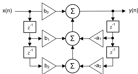
Figure 7-21. IIR H(z)
