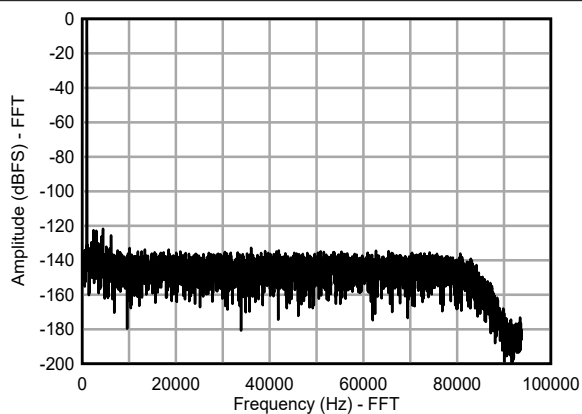
Figure 9-5. Wideband Filter Performance
